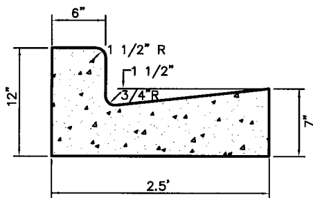
TYPICAL CURB SECTION
